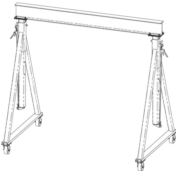
Ratchet Lever Height Adjustment
